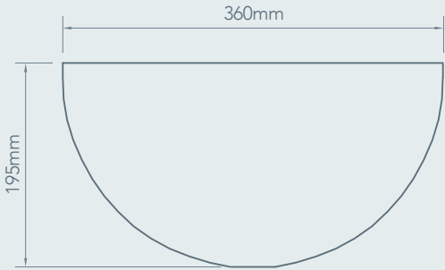
PEROSA BASIN 360mm
