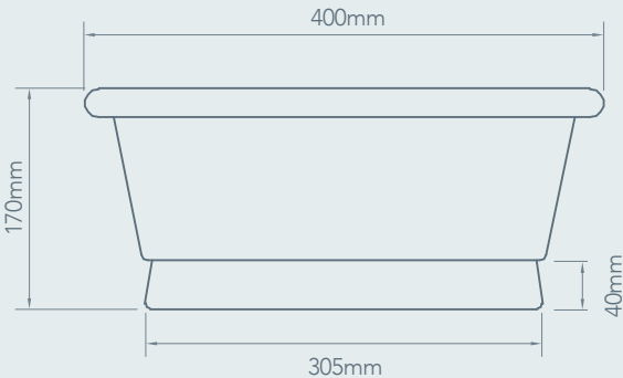
ROTUNDUS BASIN 400mm
